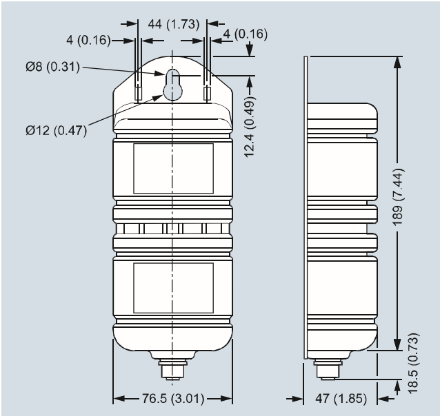
Dimensions in mm (inch), weight 2.0 kg (4.5 lb)
