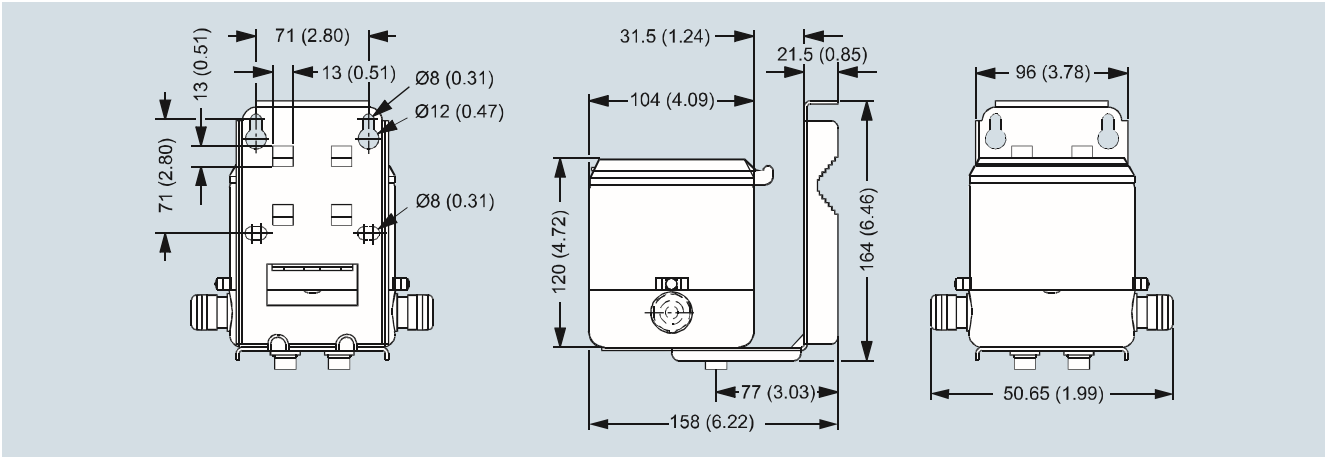
Dimensions in mm (inch), weight 3.5 kg (8 lb)
