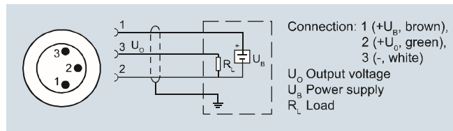
Connection with voltage output 0 ... 5 V DC (0 ... 10 V DC) and round connector
