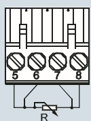
Four-wire system
